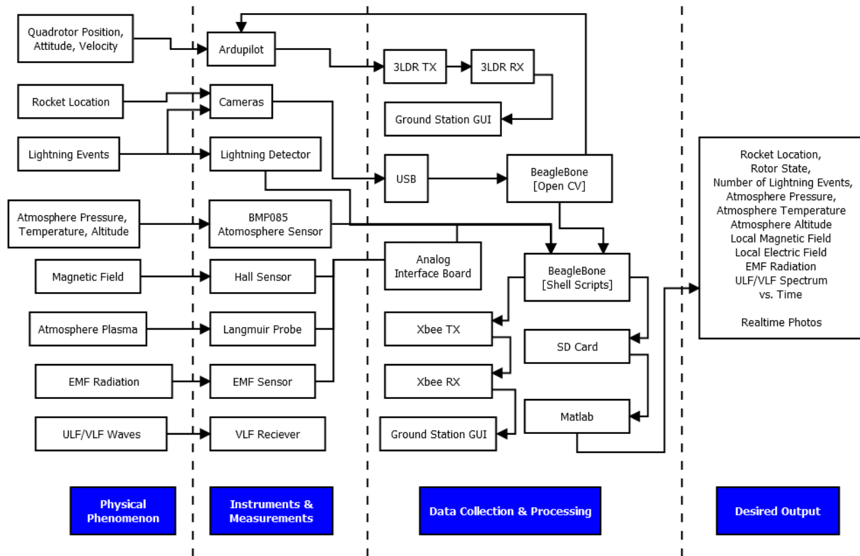
Figure 30 Conceptual Flow of Data
