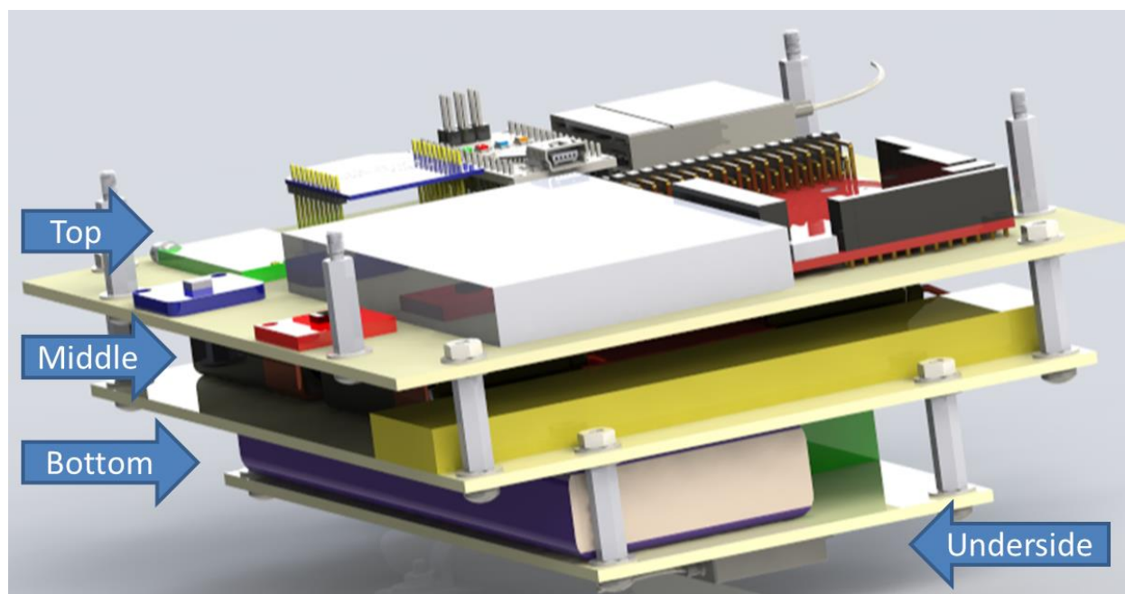
Figure 60 Placement of avionics hardware
