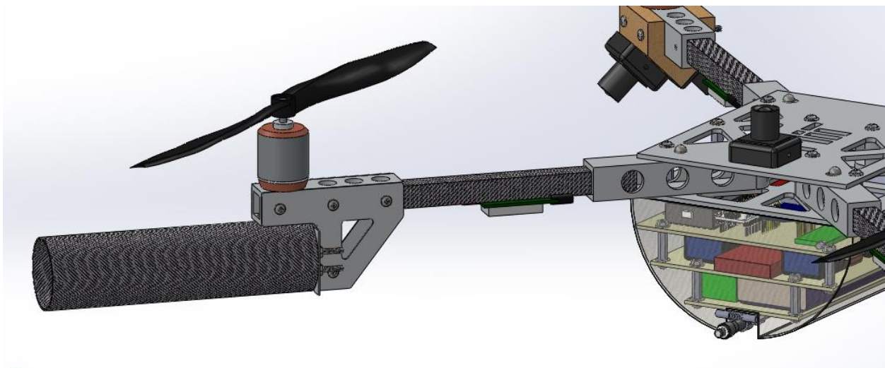
Figure 56 - The reserve parachute cannon mounted on the quadrotor's arm.
