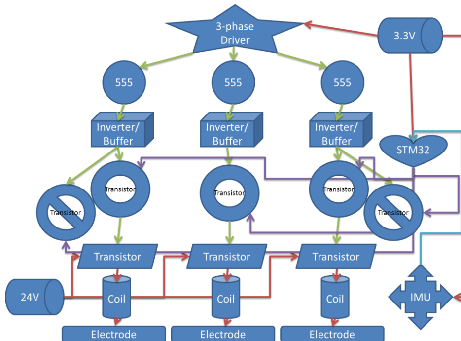
Figure 67 NIMBUS overview diagram
