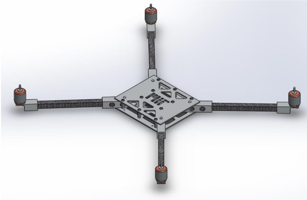
Figure 42 - Assembly Step 3
