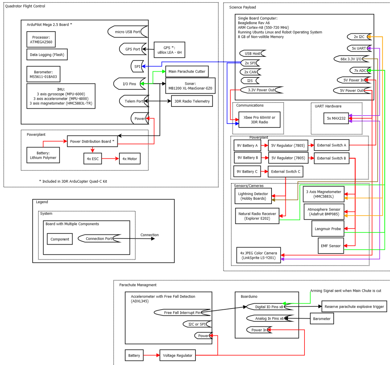
Figure 48 High-Level Avionics Interface Diagram
