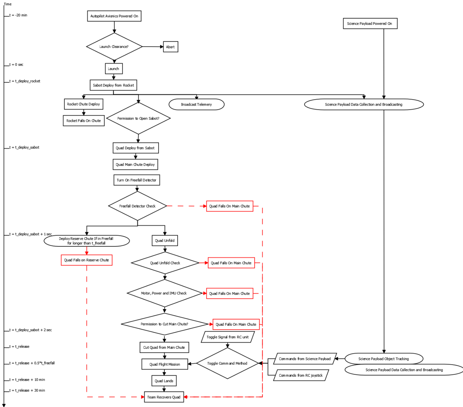
Figure 31 Concept of Operations Diagram - Time is shown on the downwards axis. Diamonds represent decisions, rectangles represent processes, rounded rectangles represent looping or continuous processes, and slanted parallelograms represent inputs. The black path indicates the intended operation; the dashed red paths indicate controlled failure modes.
