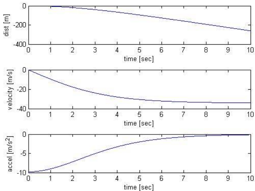
Figure 59 - A rough prediction of the quadrotor's free-fall kinematics
