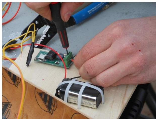
Figure 10 Rocket flight computers/batteries placement and mounting
