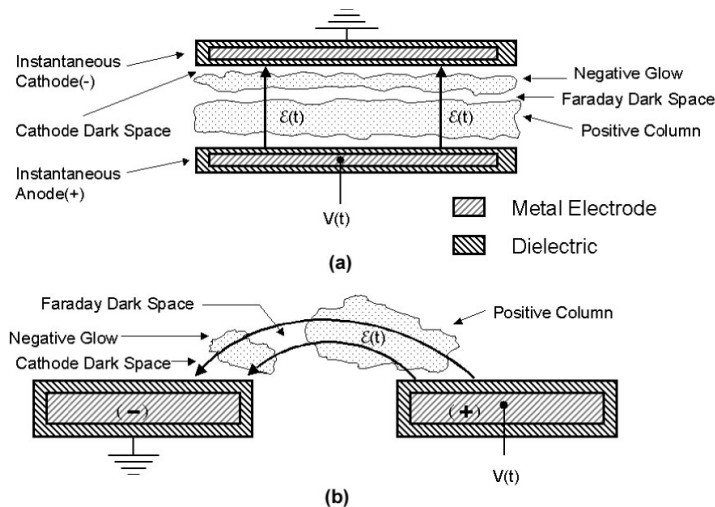
Figure 68 Electrode configuration for co-planer flat panels (J. Roth – Aerodynamic Flow Acceleration Using Electrohydrodynamic Effects)
