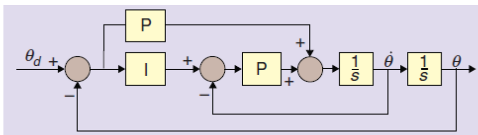
Figure 47 – ArduCopter PI + P Controller Diagram. Source: Lim et al, IEEE ROBOTICS & AUTOMATION.
