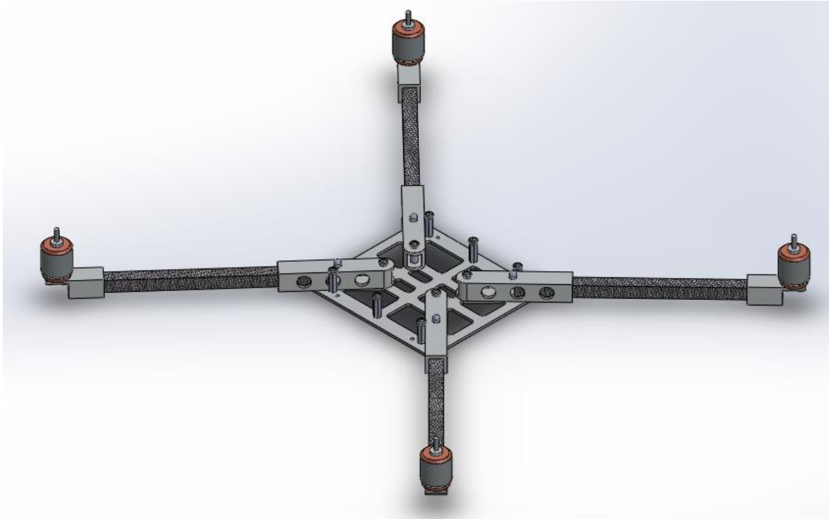
Figure 41 - Assembly Step 2
