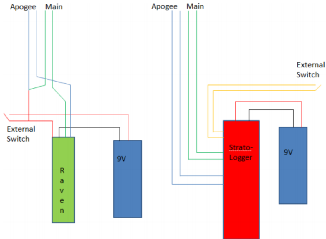
Figure 14 Rocket Avionics Wiring Diagram
