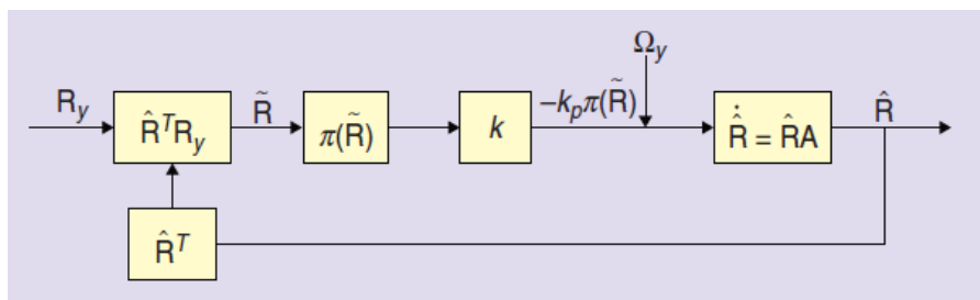
Figure 46 - Complementary Filter Diagram. R is a rotation matrix representing the attitude. Source: Lim et al, IEEE ROBOTICS & AUTOMATION.
