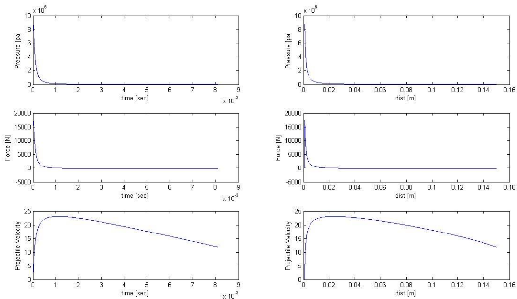
Figure 50 - Simulated pressure, force and projectile velocity from a 2 gram black powder charge
