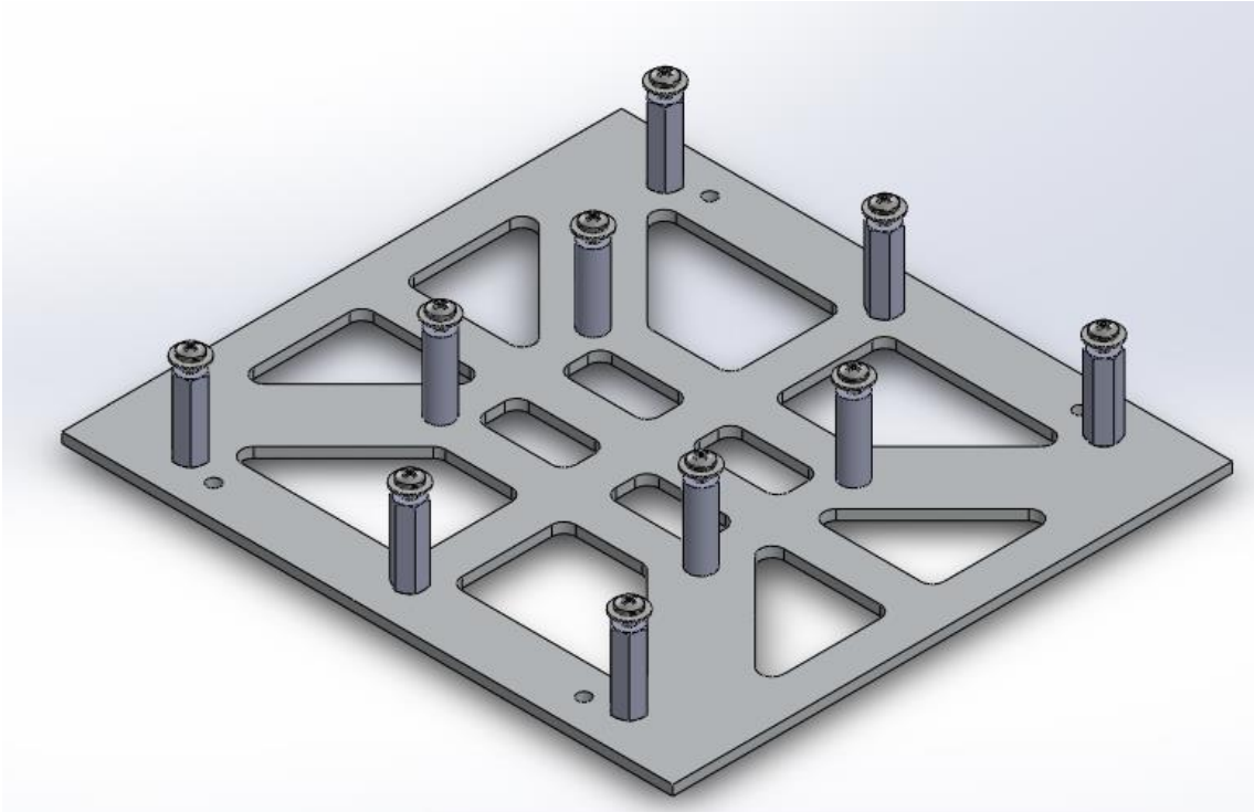
Figure 40 Assembly Step 1
