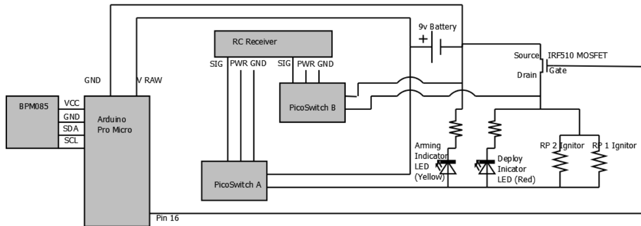
MIT Rocket Team USLI 2012-13 Reserve Parachute Deployment Circuit
