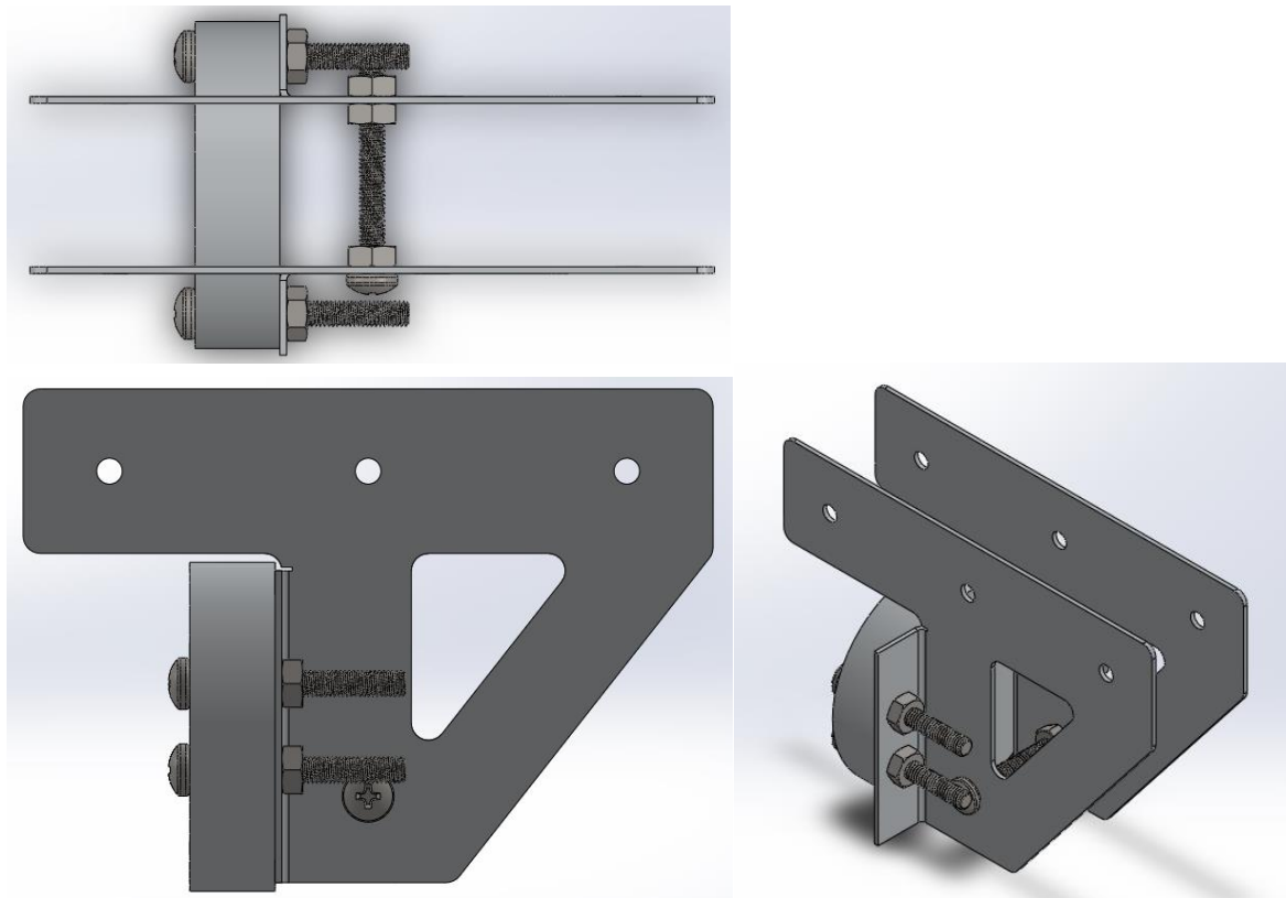
Figure 54 - The brackets bolted to the disk, in top, side and isometric view.
