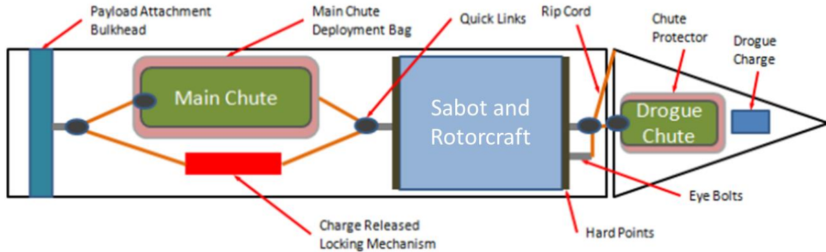
Figure 18 Payload Integration Stacking
