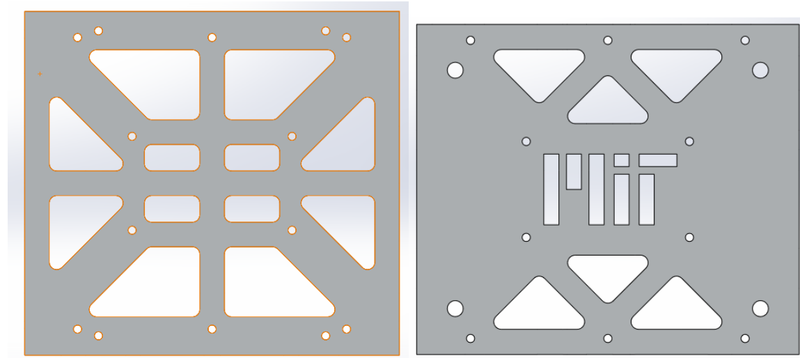
Figure 38 The bottom (left) and top (right) aluminum plates of the arm mounting block
