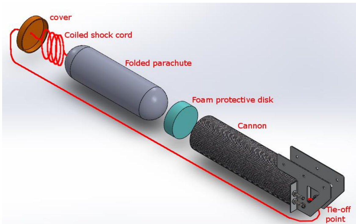
Figure 57 - Exploded view of the components packed into the reserve parachute cannon
