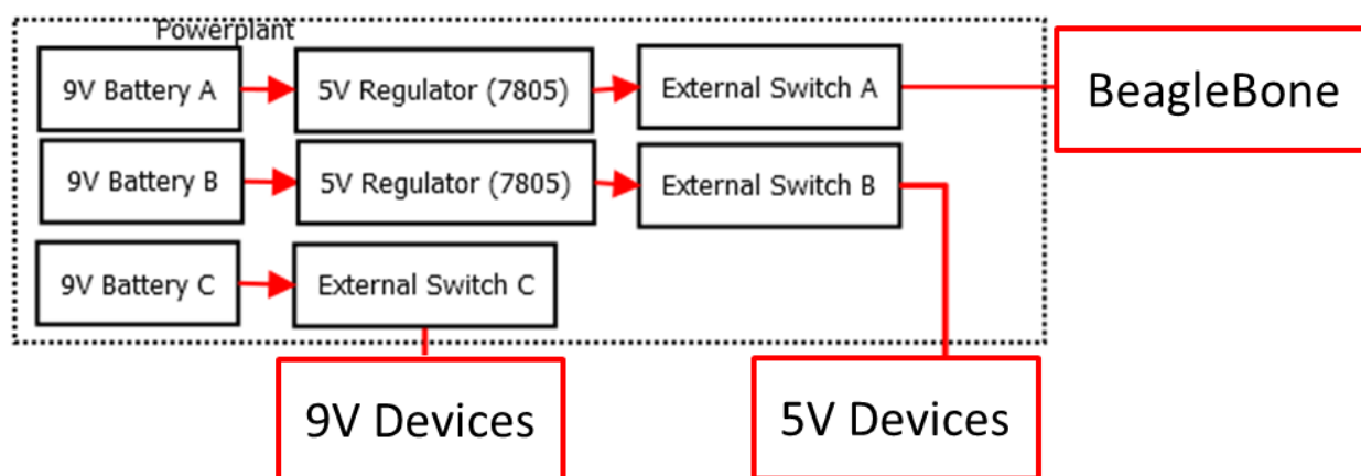
Figure 61 HALO Power Distribution Overview
