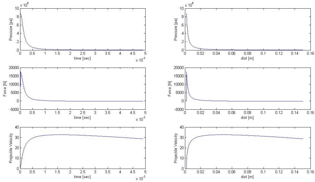
Figure 51 - Simulated pressure, force and projectile velocity from a 4 gram black powder charge
