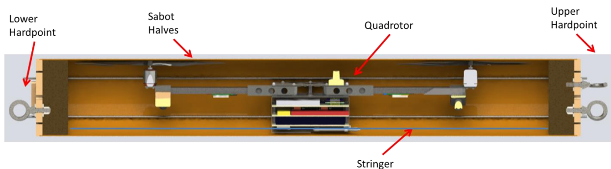
Figure 17 Sabot Overview
