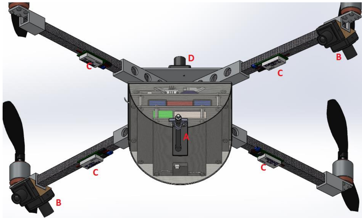
Figure 37 The Avionics tray mounted beneath the arm mounting block, covered by its Dacron® cover (transparent). The cover has a slit cut out of it for the natural radio receiver antenna (A). This view also shows the two stereo camera pairs (B), the electronic speed controllers (C), and the upward-facing camera (D).
